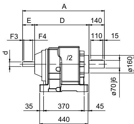
NHL 70 - GEARBOX
